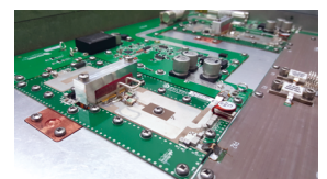
2 planar design RF pallets each of 1.7 kW
