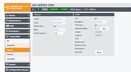
SFN audio delay GPS receiver configuration
